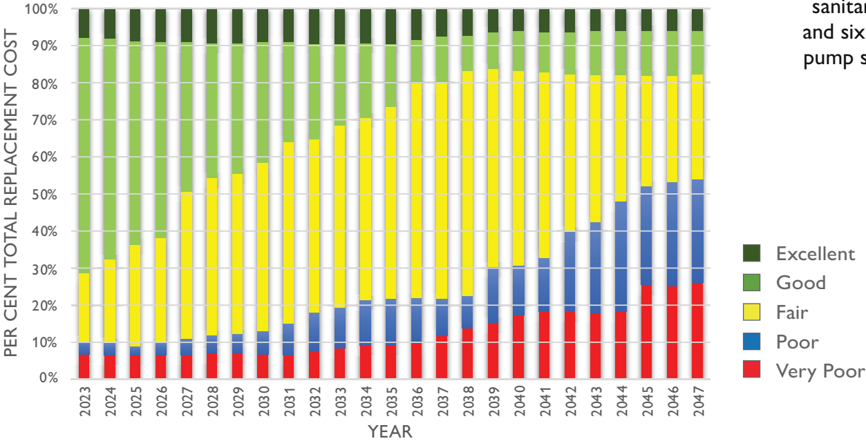
Annual performance of sanitary assets
